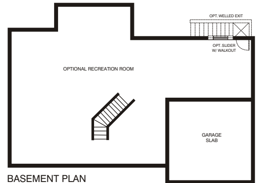
BASEMENT PLAN (Not to scale)
